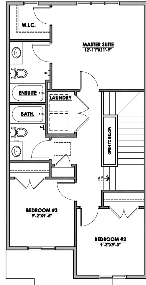
UPPER FLOOR PLAN 656 SQ.FT.
