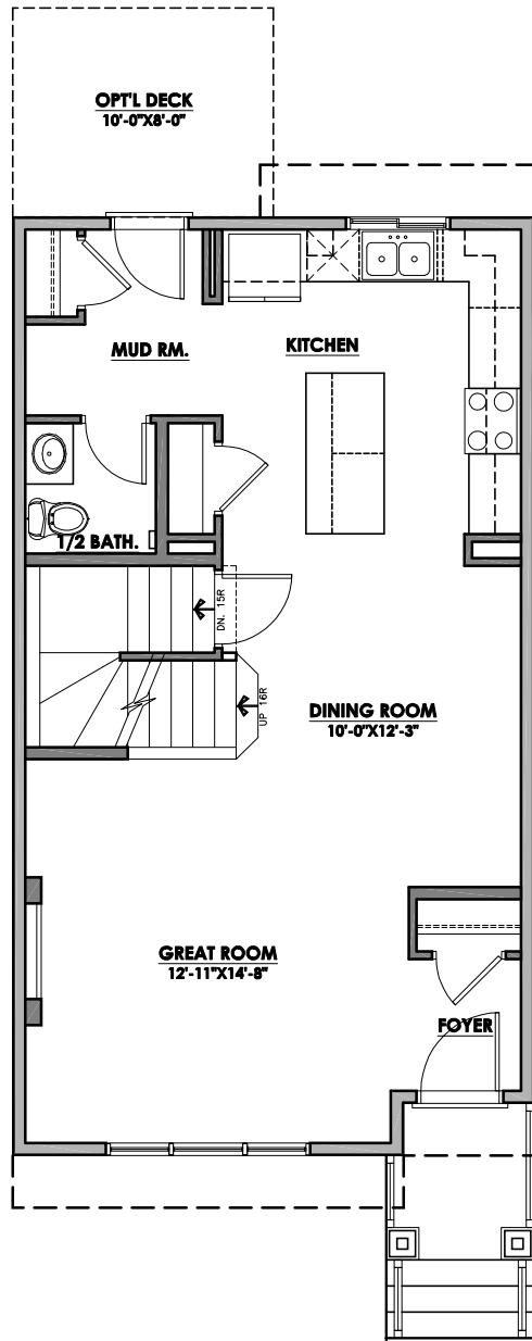
MAIN FLOOR PLAN 710 SQ.FT.
