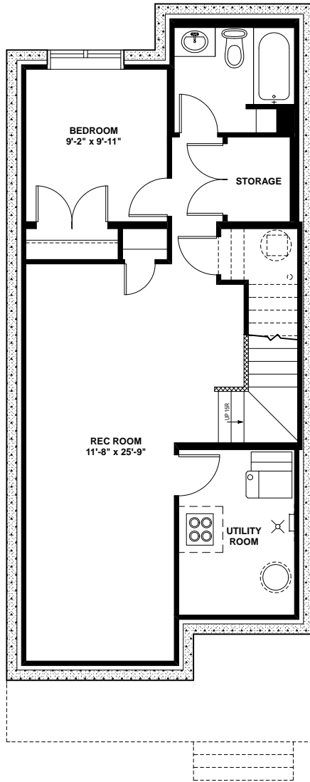
OPTIONAL BASEMENT DEVELOPMENT PLAN - 690 sq.ft.
