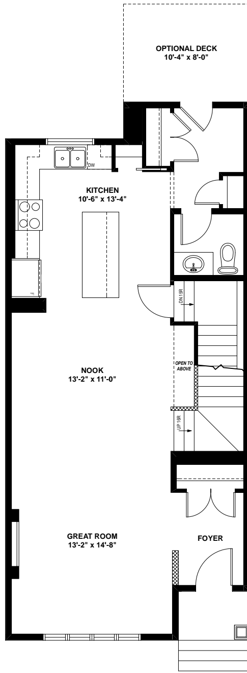
MAIN FLOOR - 827 sq. ft.
