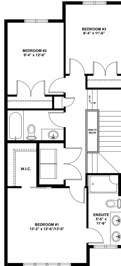
SECOND FLOOR: 754 sq. ft.
